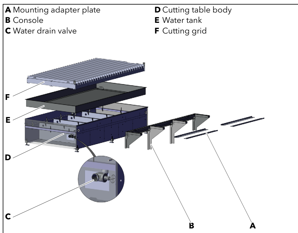
Fig. 2 Structure
