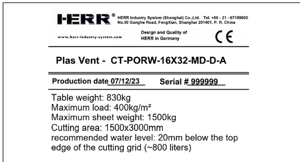
Fig. 1 HERR® Water table identification plate
